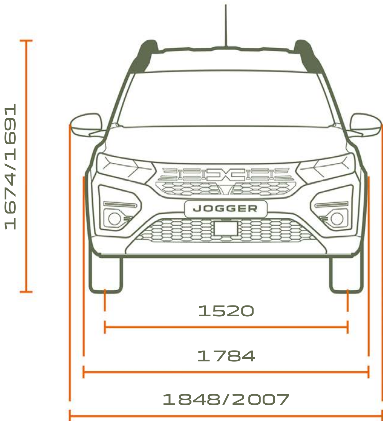
FRONT VIEW
